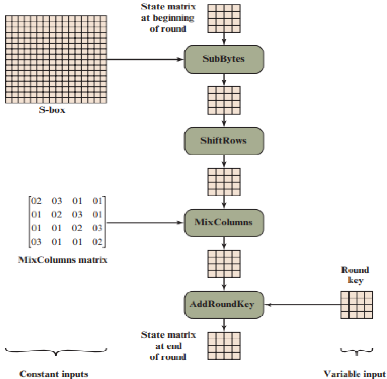
Figure 6.8 Inputs for Single AES Round
